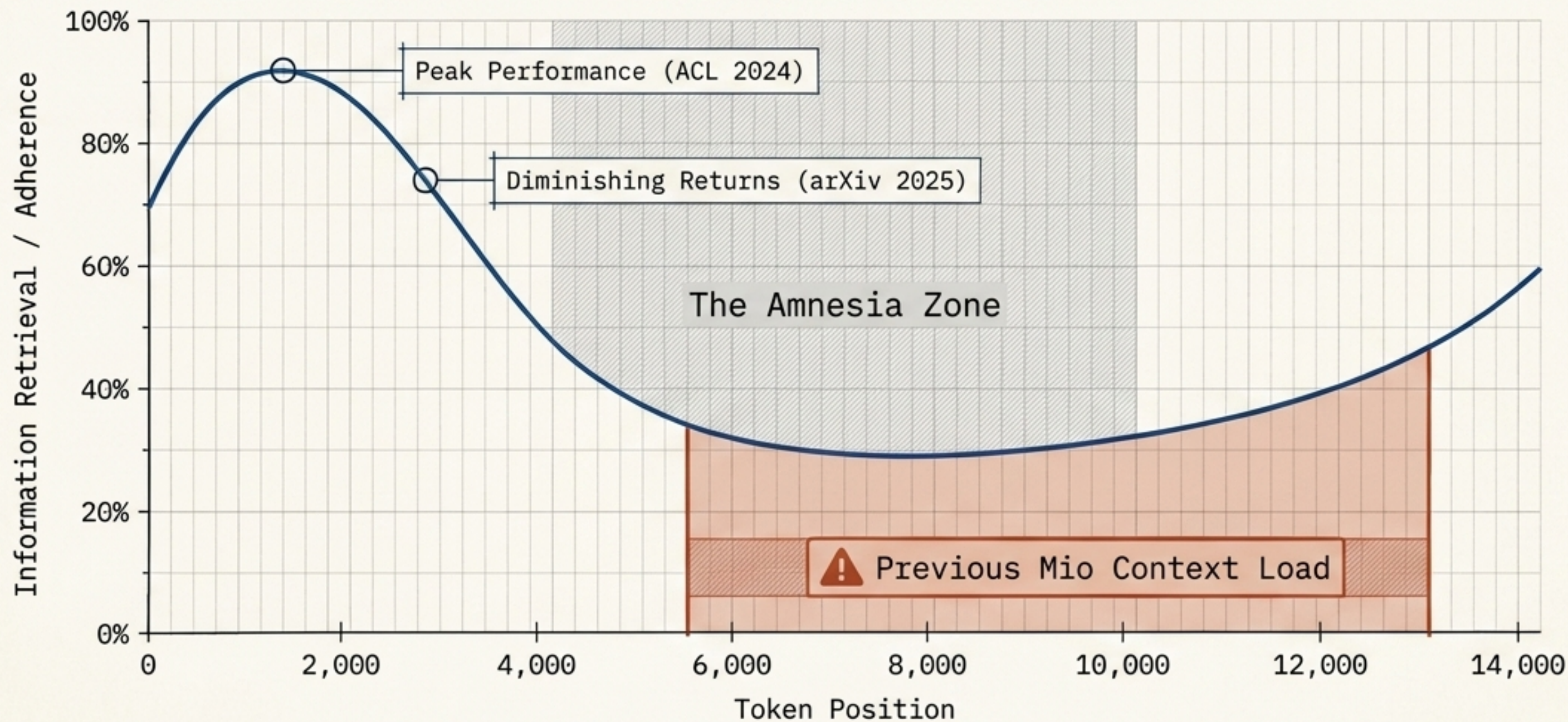
Attention Curve: "Lost in the Middle" (Liu et al.)
